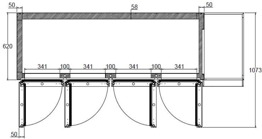
SECTION B-B
